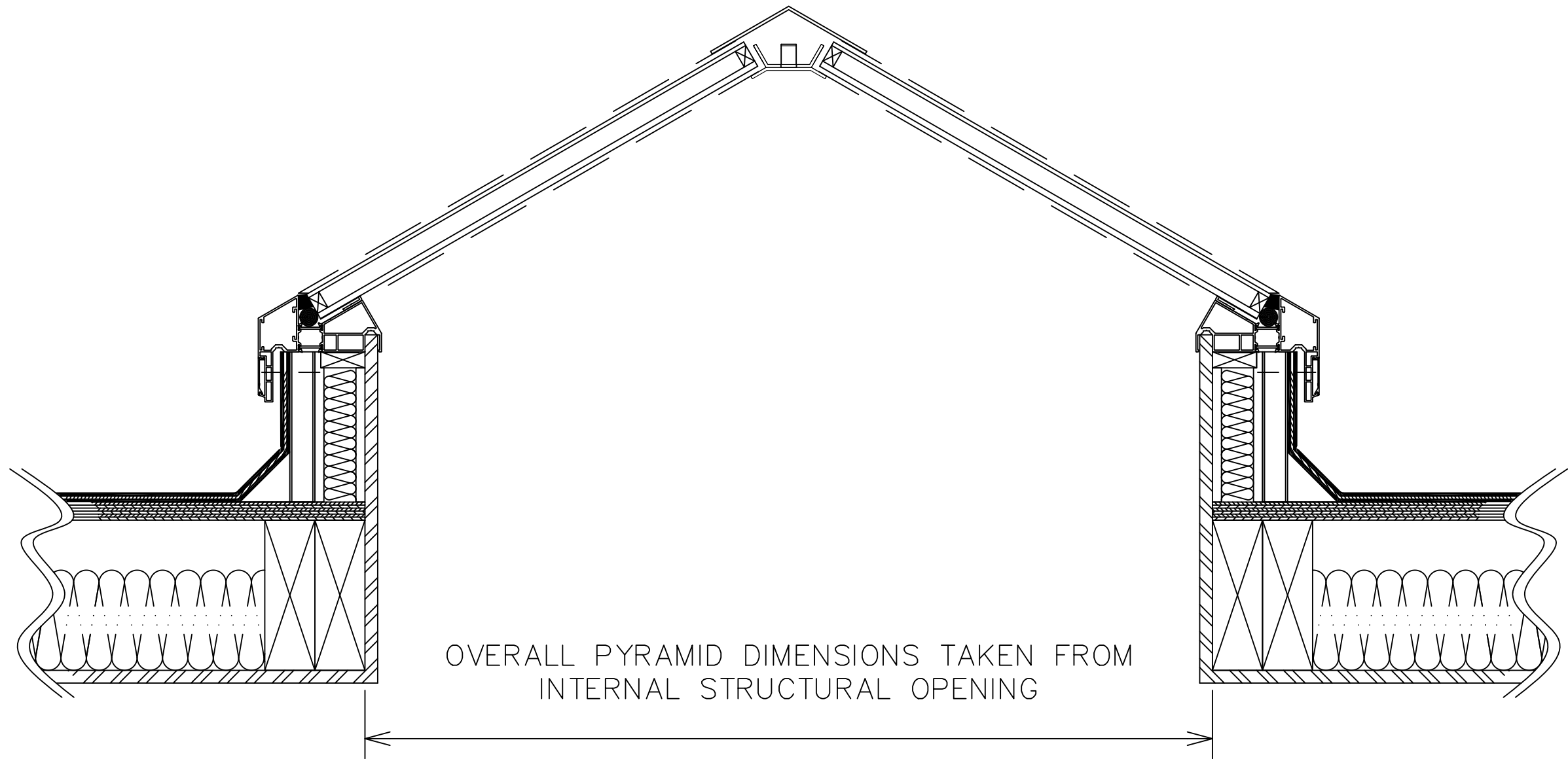
Section Through Upstand/Framework Construction
